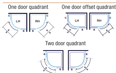
Two Door Quadrant
