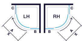
One Door Quadrant
