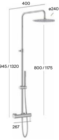
Shower column N
