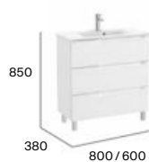
Unik compact (basin and base unit)
